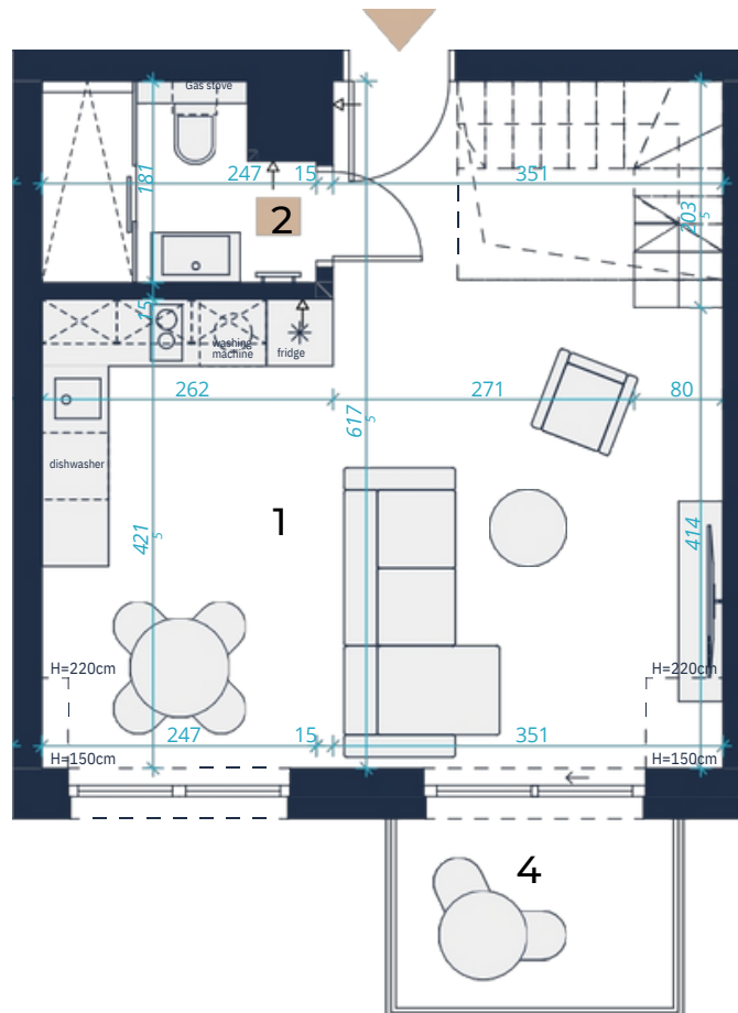
1st FLOOR
